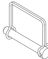
5/16" x 2 1/2" Snap Pin {1 Piece}
