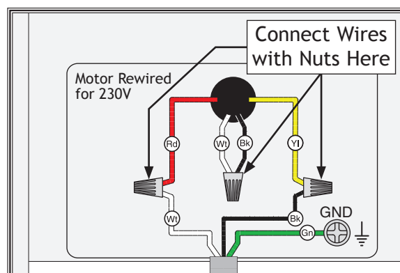
Figure 7. Motor rewired for 230V.
