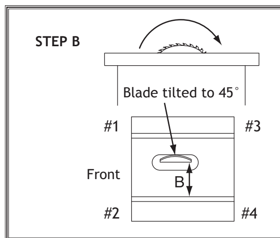
Figure 110. Shim procedure diagram B.
