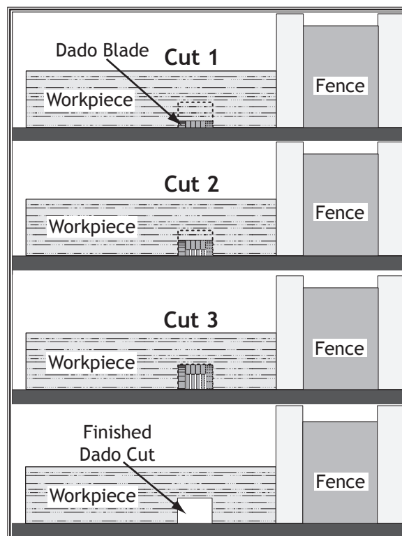
Figure 63. Example of dado being cut with multiple light cuts, instead of one deep cut.
