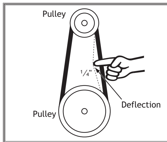
Figure 125. Checking belt tension.
