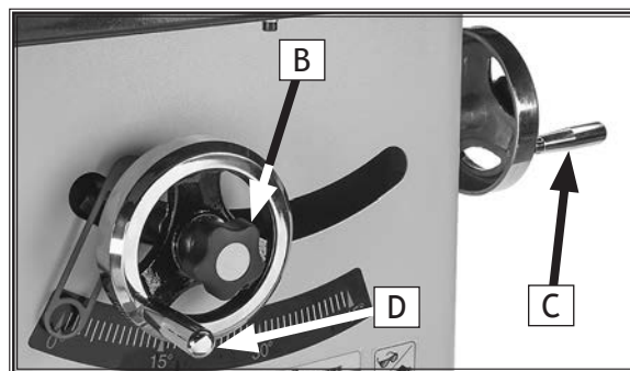
Figure 2. Blade adjustment handwheels and locks.
