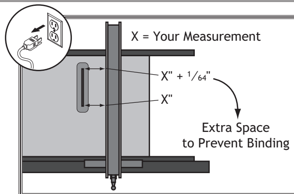
Figure 118. Adjusting fence with a \frac{1}{64} " offset.
