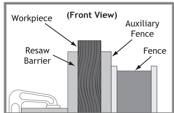
Figure 76. Example illustration of a resaw setup.
