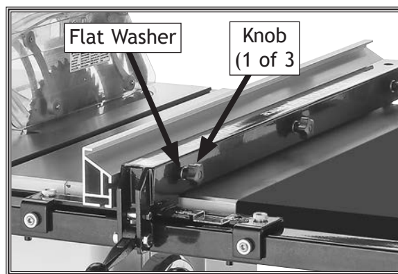
Figure 74. Location of knobs and flat washers securing fence to fence tube.
