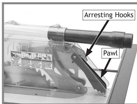
Figure 53. Pawls in resting position.
