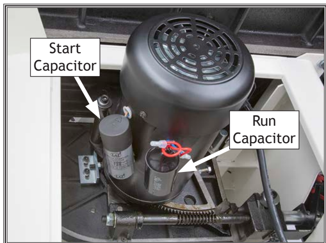
Figure 126. Motor capacitors.
