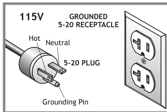
Figure 4. NEMA 5-20 plug & receptacle.
