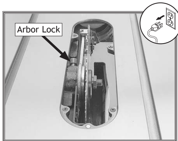
Figure 44. Location of arbor lock.
