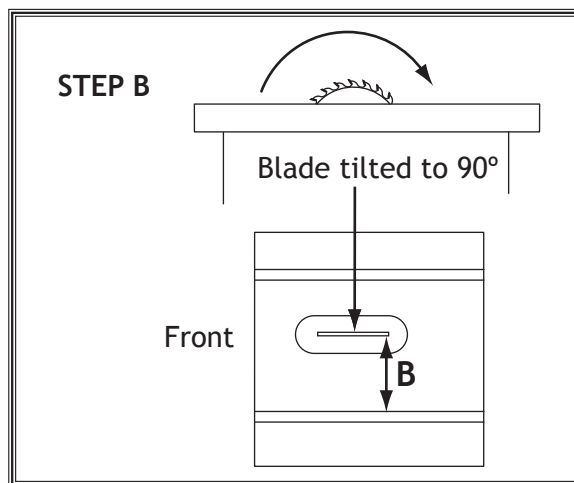
Figure 107. Making second slot-to-blade measurement at 90°.
