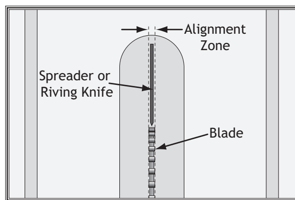
Figure 112. Spreader/riving knife alignment zone.
