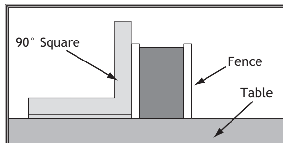
Figure 116. Checking if fence is square to table.
