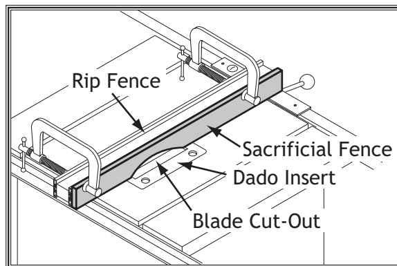
Figure 67. Example of sacrificial fence.
