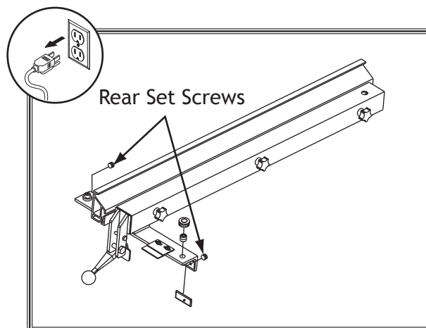
Figure 114. Location of screws used to adjust fence parallelism and clamping pressure.
