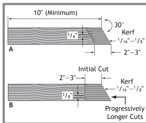
Figure 78. Patterns for making featherboards.
