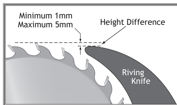
Figure 55. Example of height difference between riving knife and blade.
