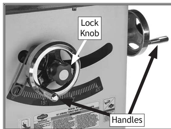
Figure 15. Handwheels installed.
