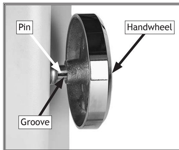
Figure 14. Handwheel installed on shaft pin.
