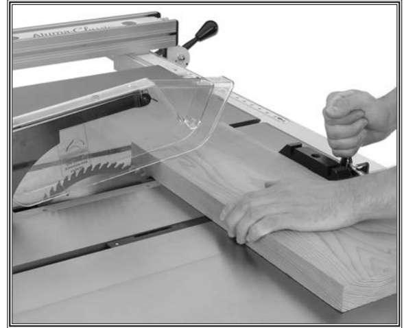
Figure 59. Typical crosscutting operation.
