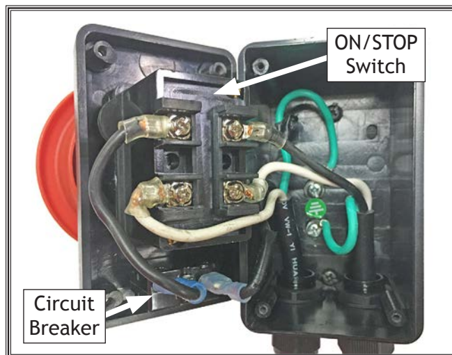
Figure 128. Switch box components.
