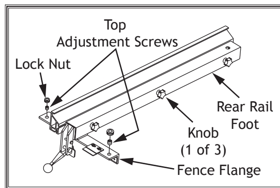
Figure 115. Fence components used to adjust fence height and squareness to table.
