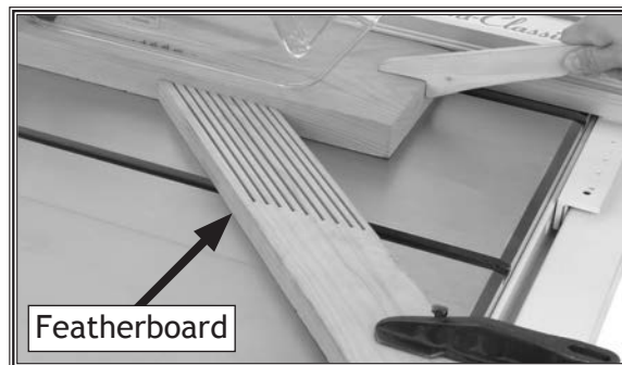
Figure 58. Typical ripping operation.
