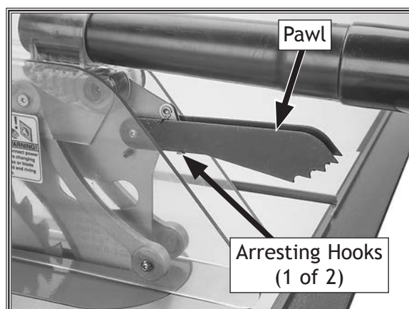
Figure 54. Pawls disabled.
