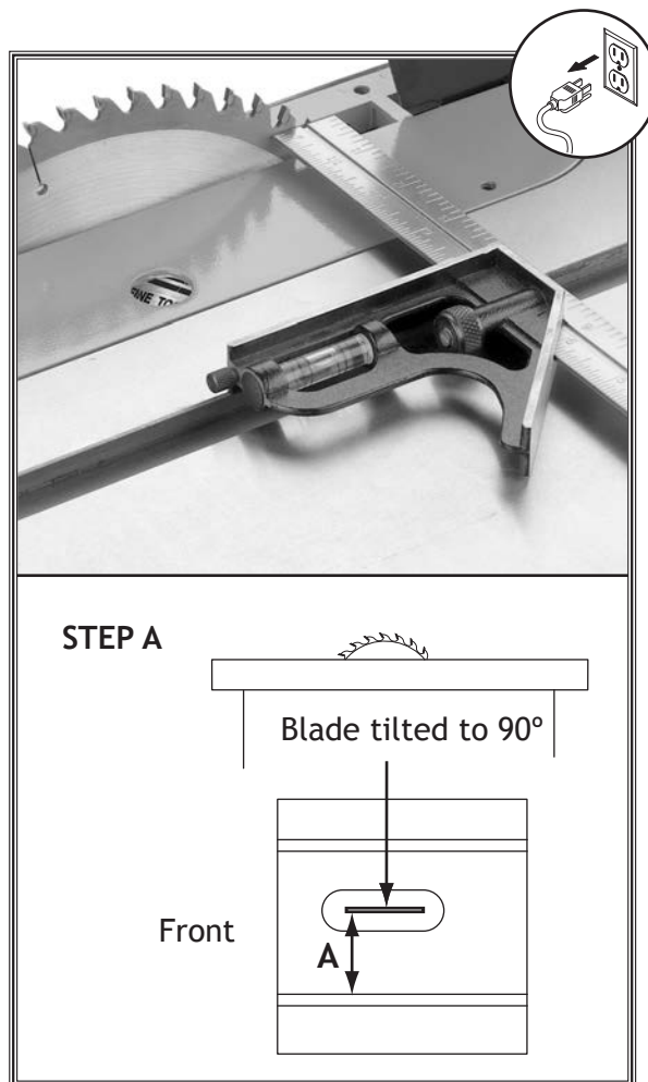
Figure 106. Making first slot-to-blade measurement at 90°.
