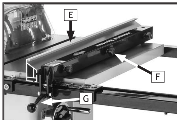
Figure 3. Location of fence controls.
