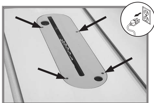
Figure 120. Location of table/dado insert holes with adjustment screws.
