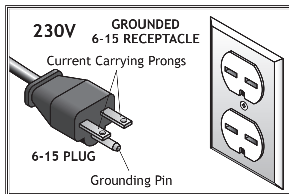
Figure 5. NEMA 6-15 plug & receptacle.
