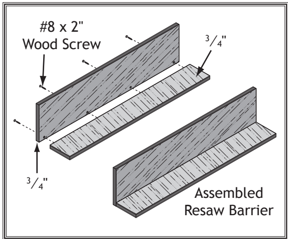
Figure 72. Resaw barrier.
