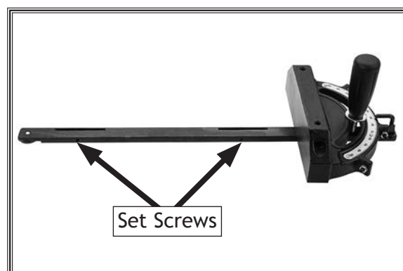
Figure 123. Set screws for adjusting miter bar tightness in miter slot.
