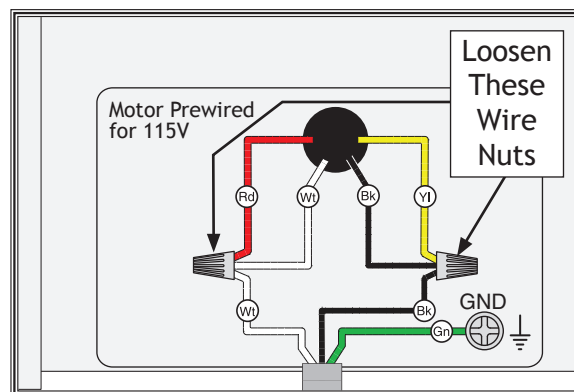
Figure 6. Motor prewired for 115V.
