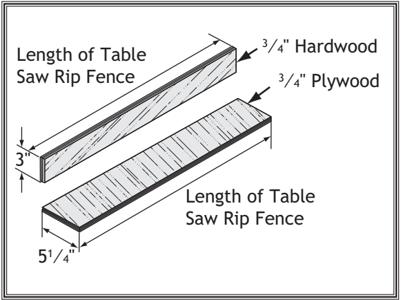
Figure 90. Auxiliary fence dimension.
