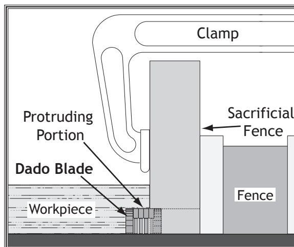
Figure 68. Rabbet cutting.
