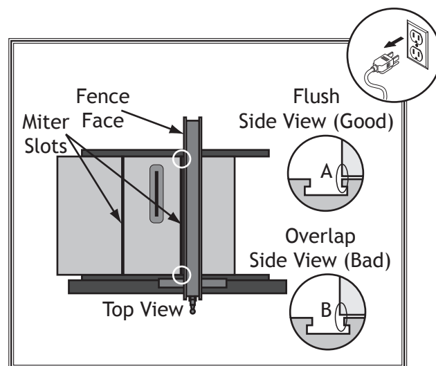
Figure 117. Example of aligning fence to miter slot.
