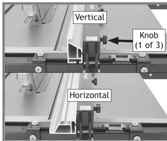
Figure 57. Rip fence positions.
