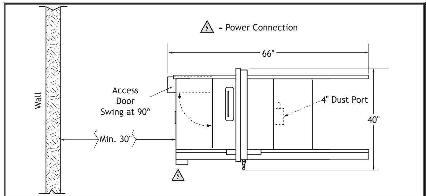
Figure 13. Working clearances.
