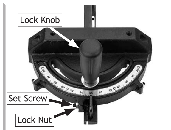
Figure 121. Screws for adjusting miter stops.
