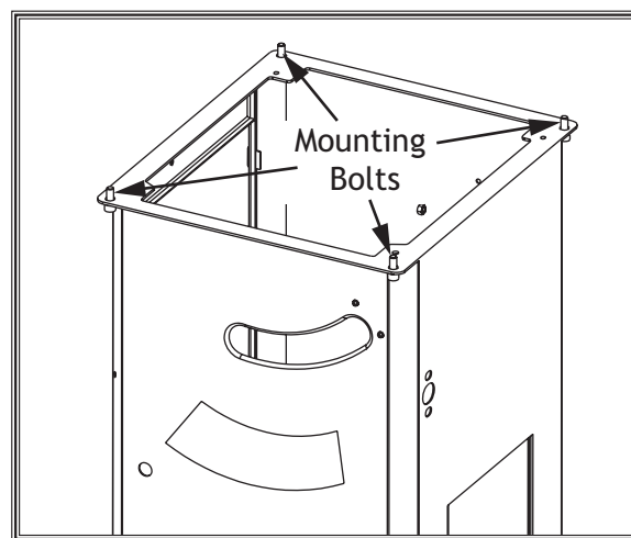
Figure 108. Location of table mounting bolts (table omitted for clarity).
