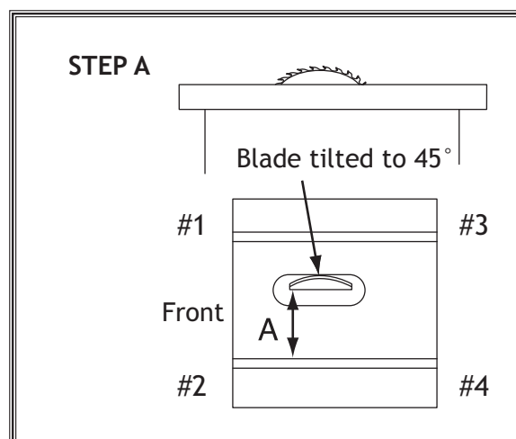
Figure 109. Shim procedure diagram A.
