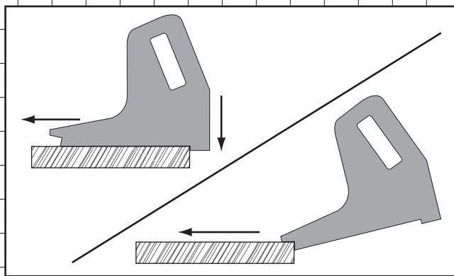
Figure 87. Side view of a push block in use.
