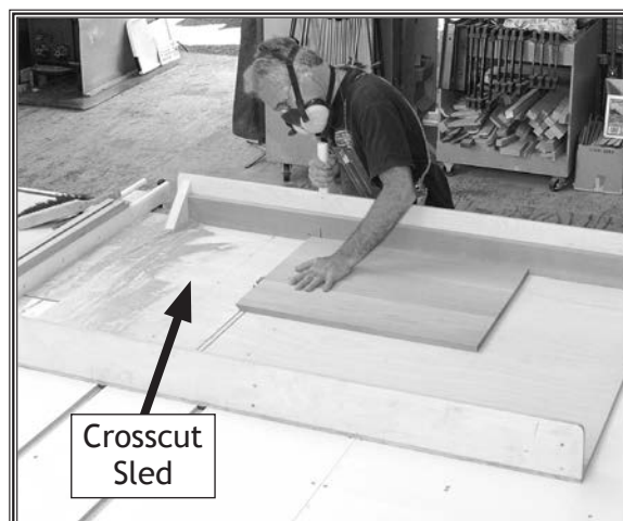
Figure 97. Example of a crosscut sled.
