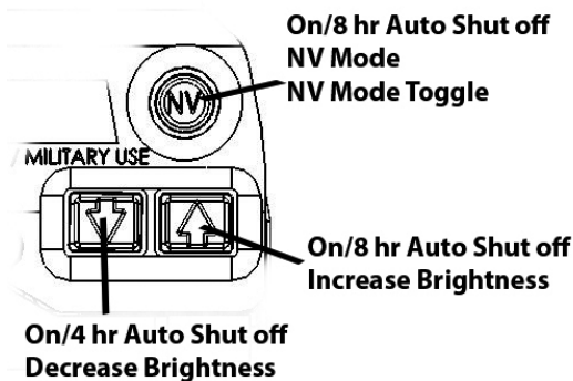
Fig 4: Pushbutton interface
