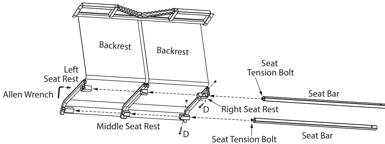
FIG. 5 STEP 8. Thread the seat tension bolts completely into the seat bars . Insert the seat bars through the seat rests and secure using (2) 1/4" x 1 3/4" hex bolts [D] and (2) 1/4" nylock nuts. Then, using the allen wrench turn the seat tension bolts counterclockwise until the seat is taught.
