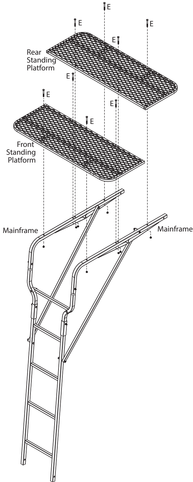
FIG. 3 STEP 5. Using (8) 1/4" x 2 1/4" [E] and (8) 1/4" nylock nuts attach the front and rear standing platforms to the mainframes .
